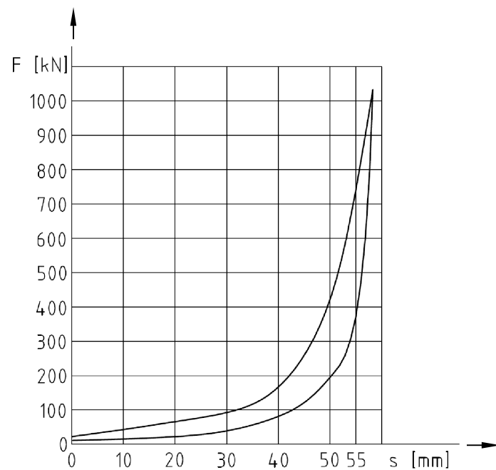
Static characteristic
